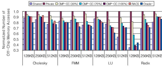
Figure 6. Normalized number of off-chip memory accesses (base case: private scheme).
