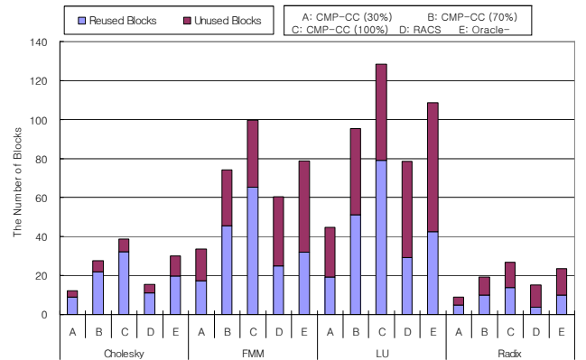
Figure 5. The number of unused blocks and reused blocks of each scheme.
